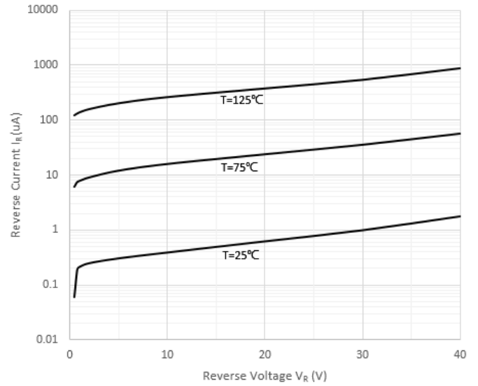
Reverse Characteristics
